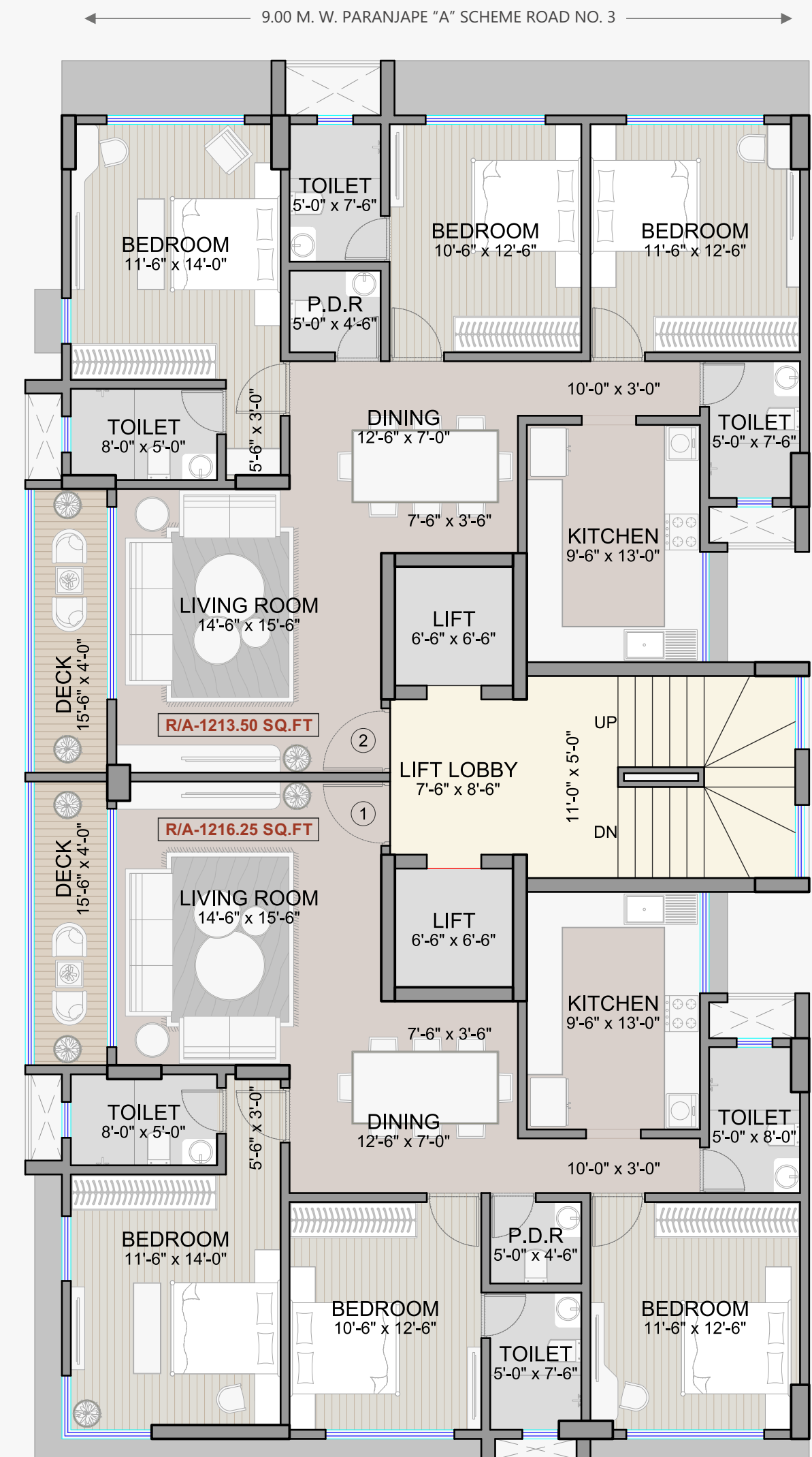
TYPICAL FLOOR PLAN (1ST, 3RD-6TH FLOOR)
